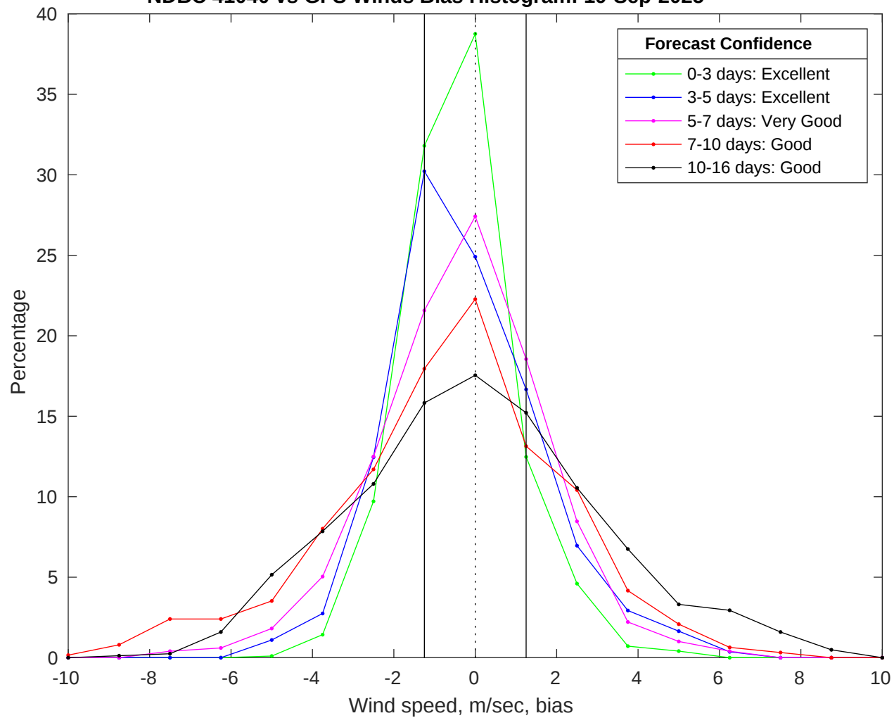
NDBC 41040 vs GFS Winds Bias Histogram: 19-Sep-2025
