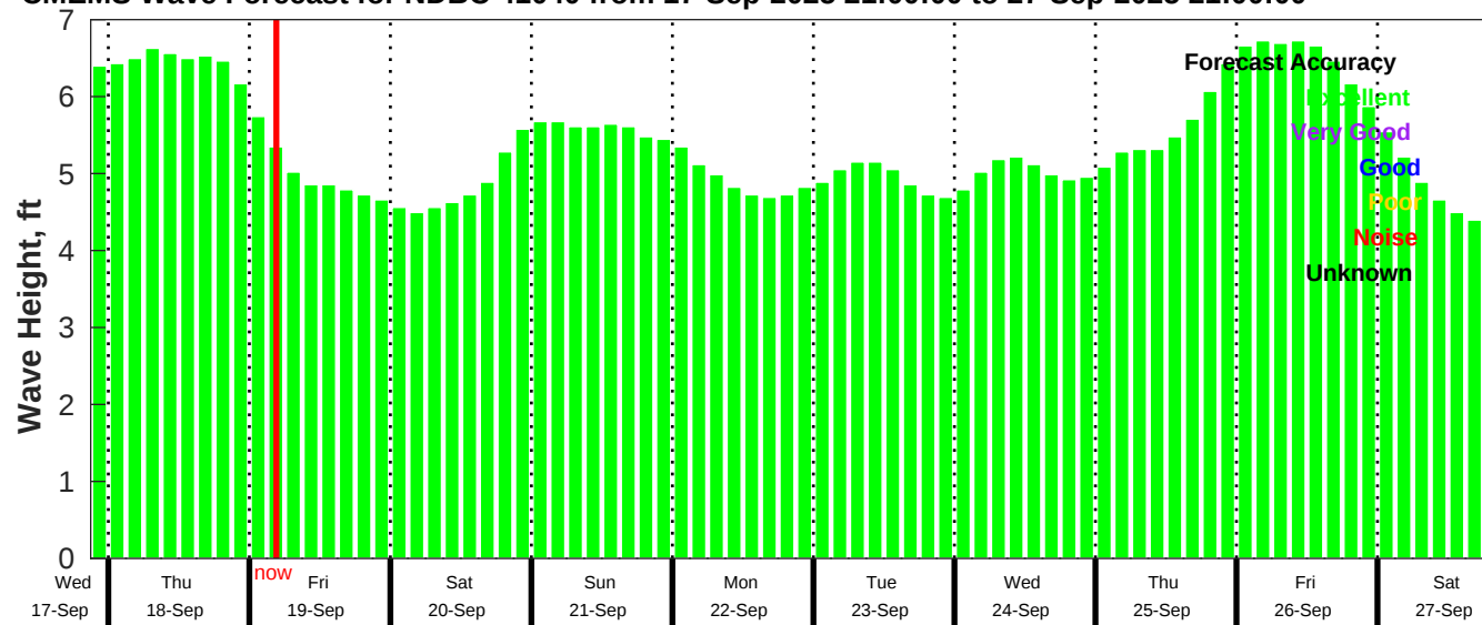
CMEMS Wave Forecast for NDBC 41040 from 17-Sep-2025 21:00:00 to 27-Sep-2025 21:00:00
