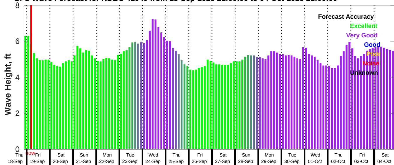
GFS Wave Forecast for NDBC 41040 from 18-Sep-2025 21:00:00 to 04-Oct-2025 21:00:00
