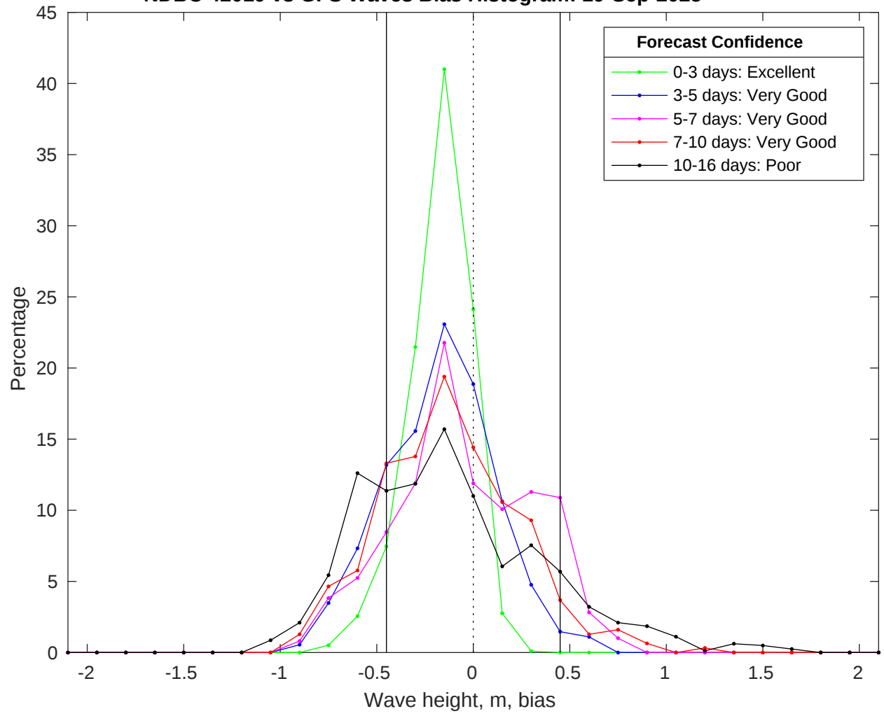
NDBC 42019 vs GFS Waves Bias Histogram: 19-Sep-2025
