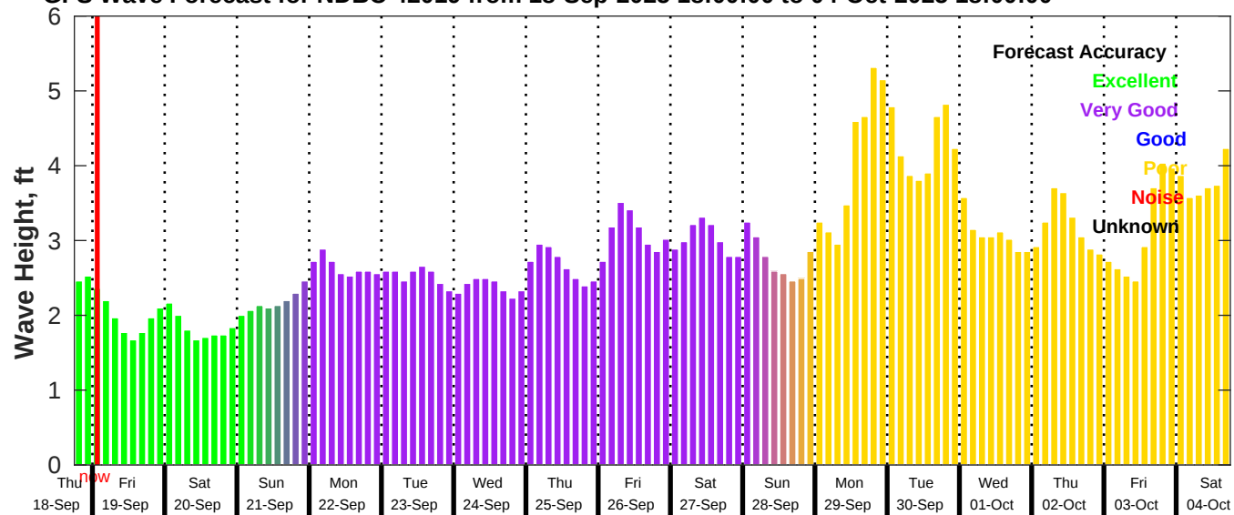
GFS Wave Forecast for NDBC 42019 from 18-Sep-2025 18:00:00 to 04-Oct-2025 18:00:00
