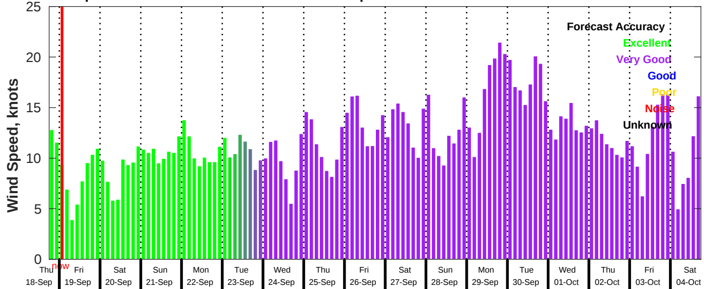
GFS Wind Speed Forecast for NDBC 42019 from 18-Sep-2025 18:00:00 to 04-Oct-2025 18:00:00
