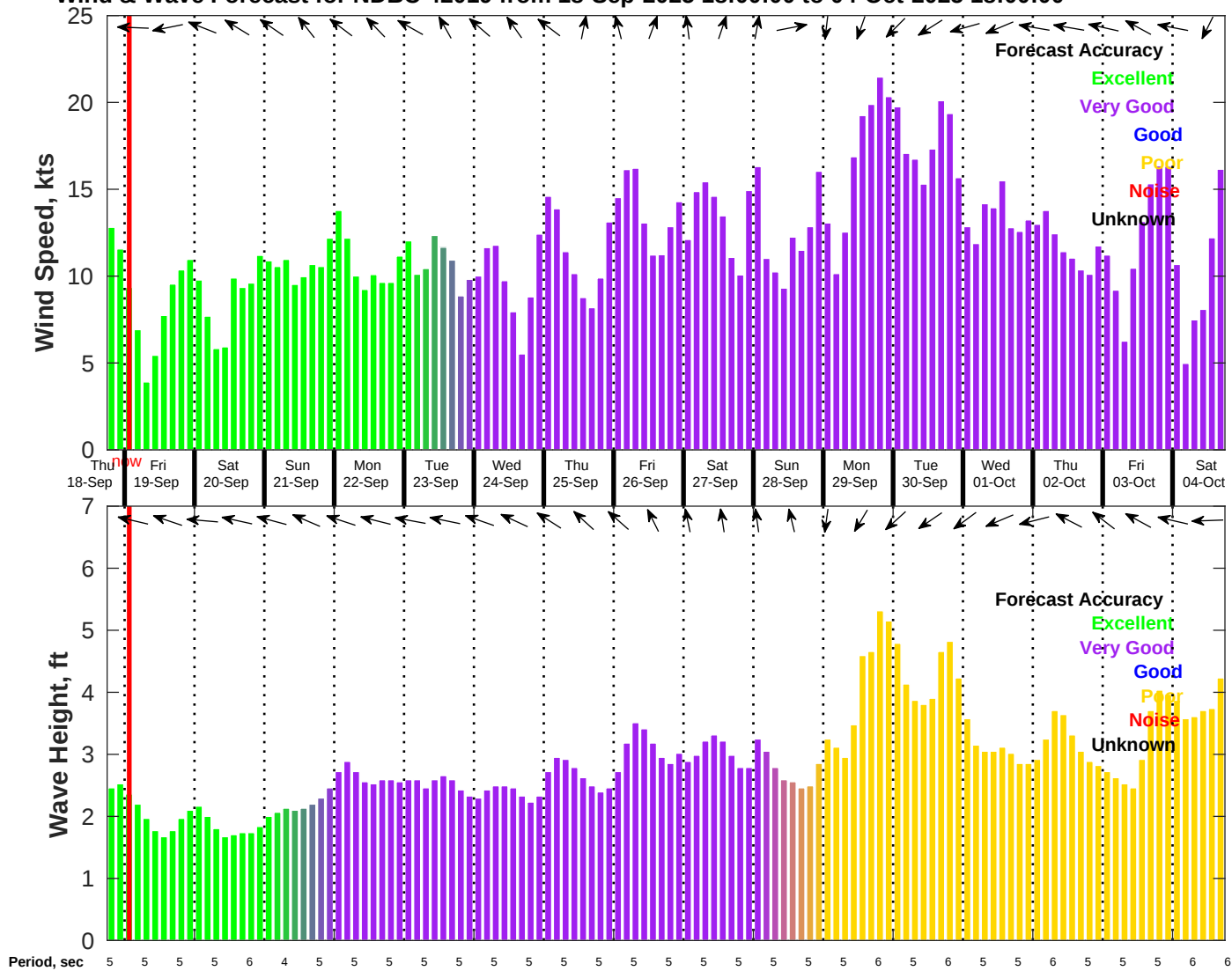
Wind & Wave Forecast for NDBC 42019 from 18-Sep-2025 18:00:00 to 04-Oct-2025 18:00:00
