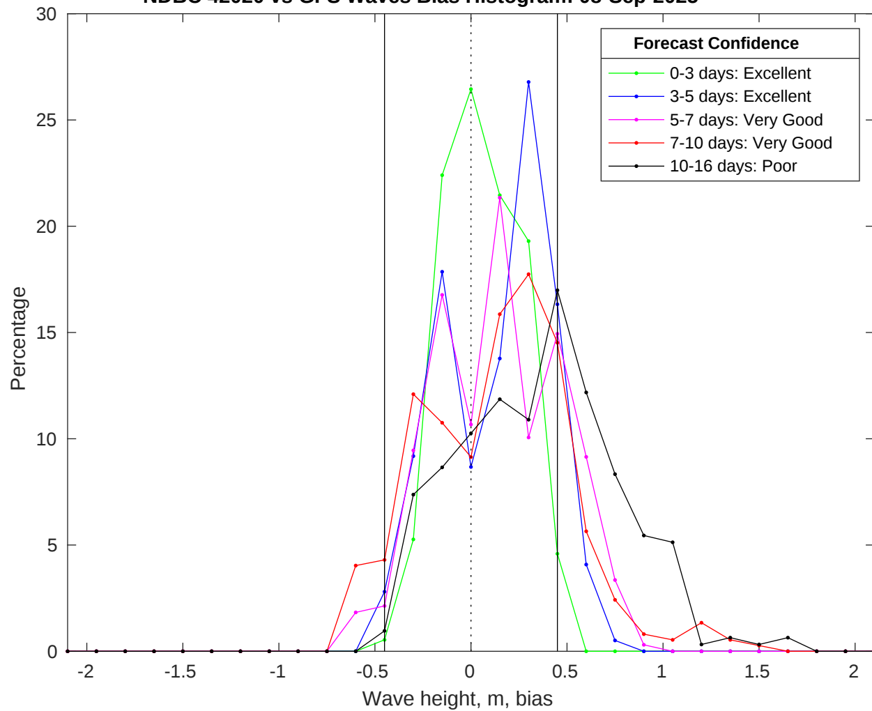
NDBC 42020 vs GFS Waves Bias Histogram: 08-Sep-2025
