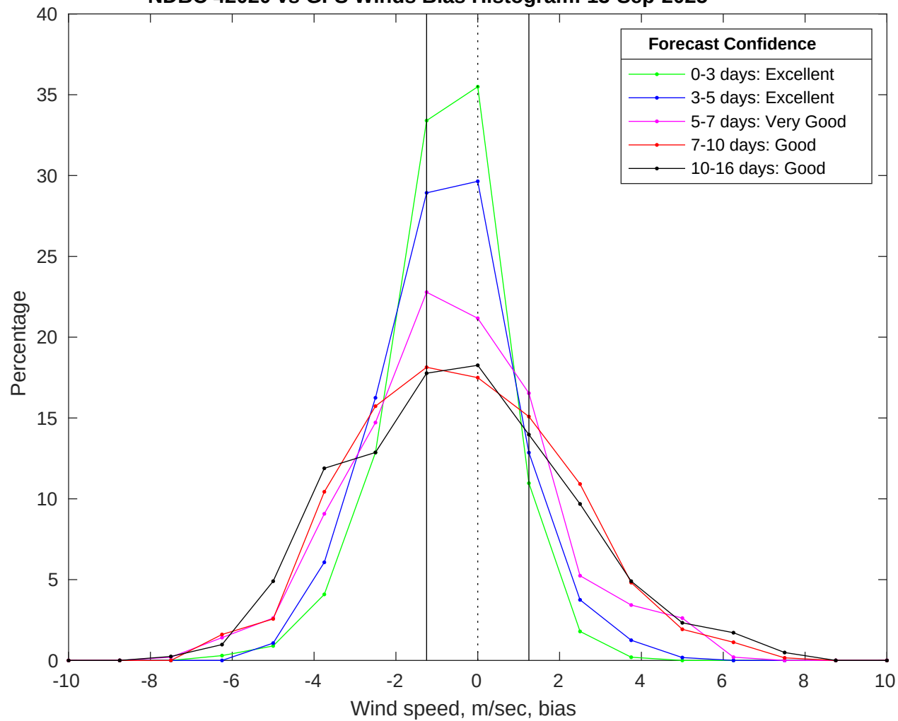
NDBC 42020 vs GFS Winds Bias Histogram: 13-Sep-2025
