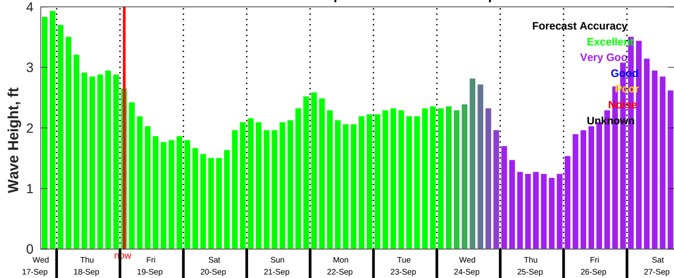
CMEMS Wave Forecast for NDBC 42020 from 17-Sep-2025 18:00:00 to 27-Sep-2025 18:00:00
