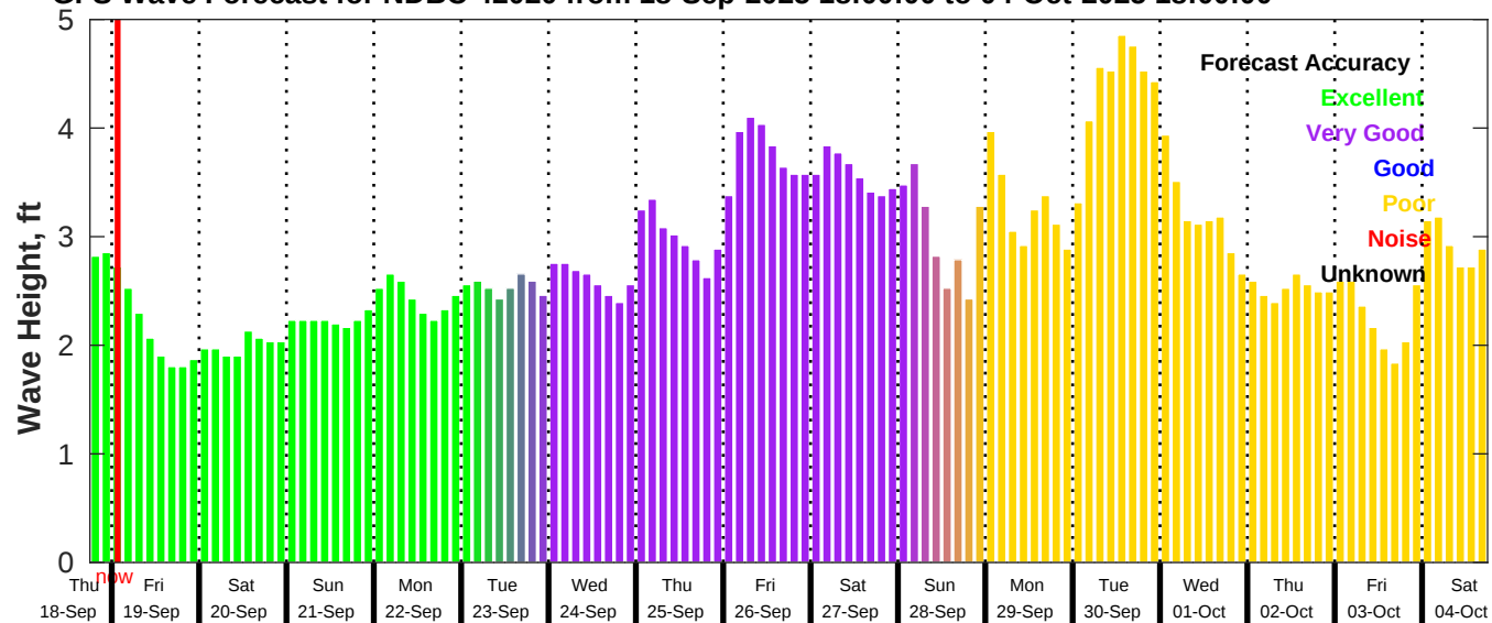
GFS Wave Forecast for NDBC 42020 from 18-Sep-2025 18:00:00 to 04-Oct-2025 18:00:00
