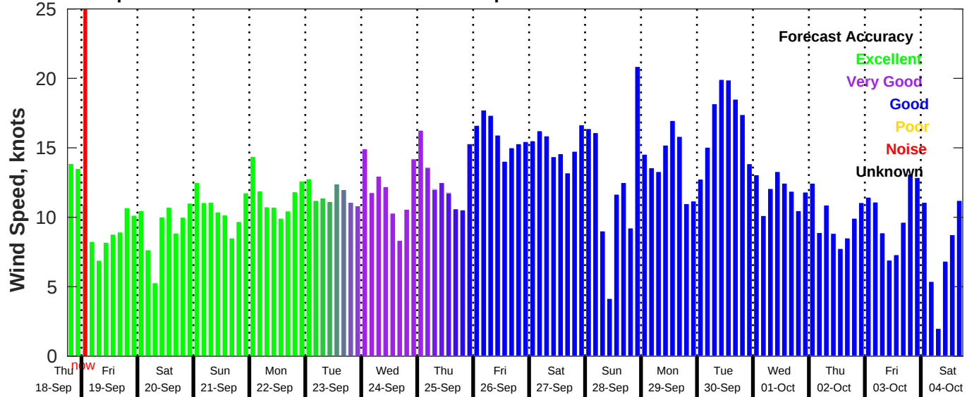
GFS Wind Speed Forecast for NDBC 42020 from 18-Sep-2025 18:00:00 to 04-Oct-2025 18:00:00
