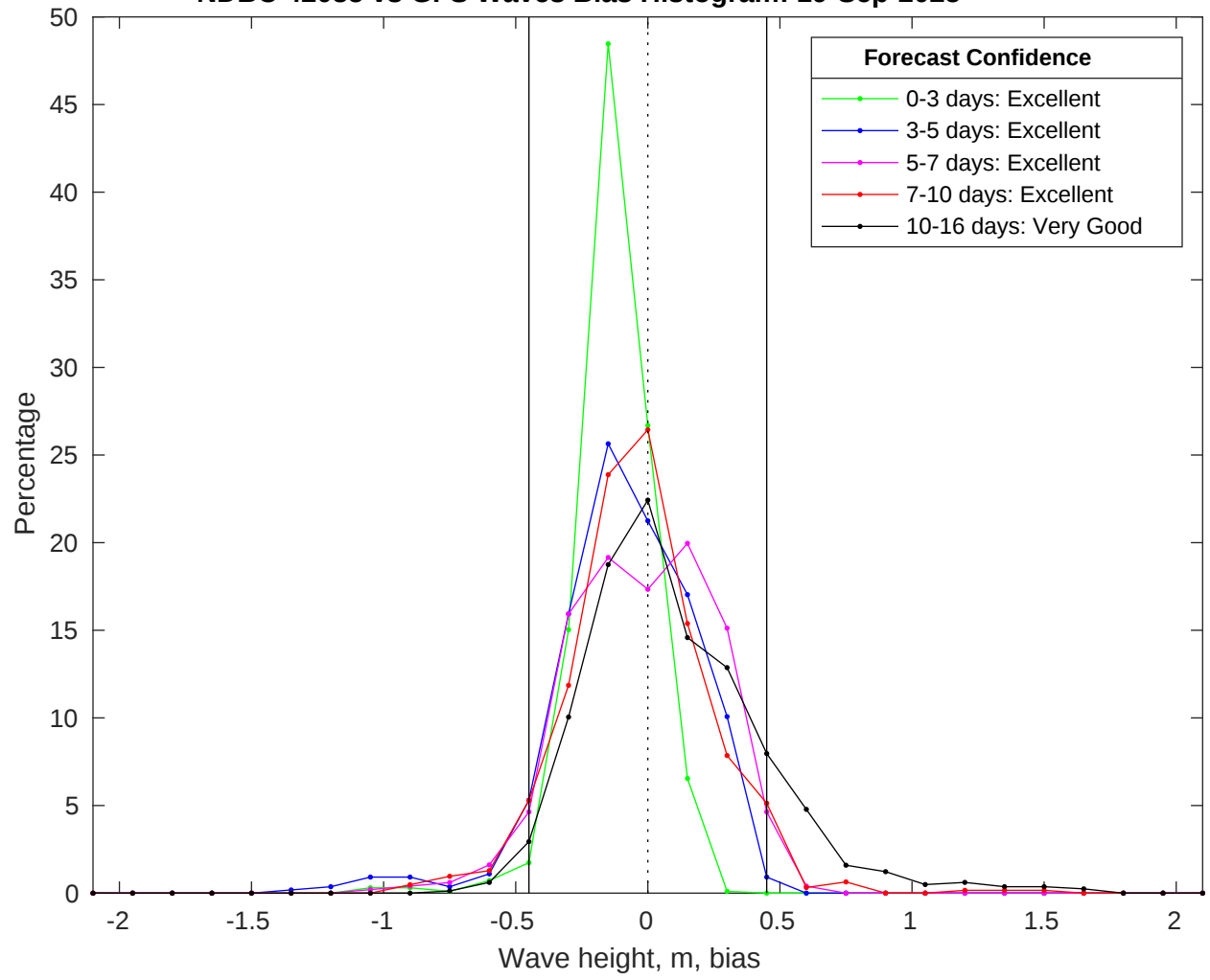
NDBC 42035 vs GFS Waves Bias Histogram: 19-Sep-2025
