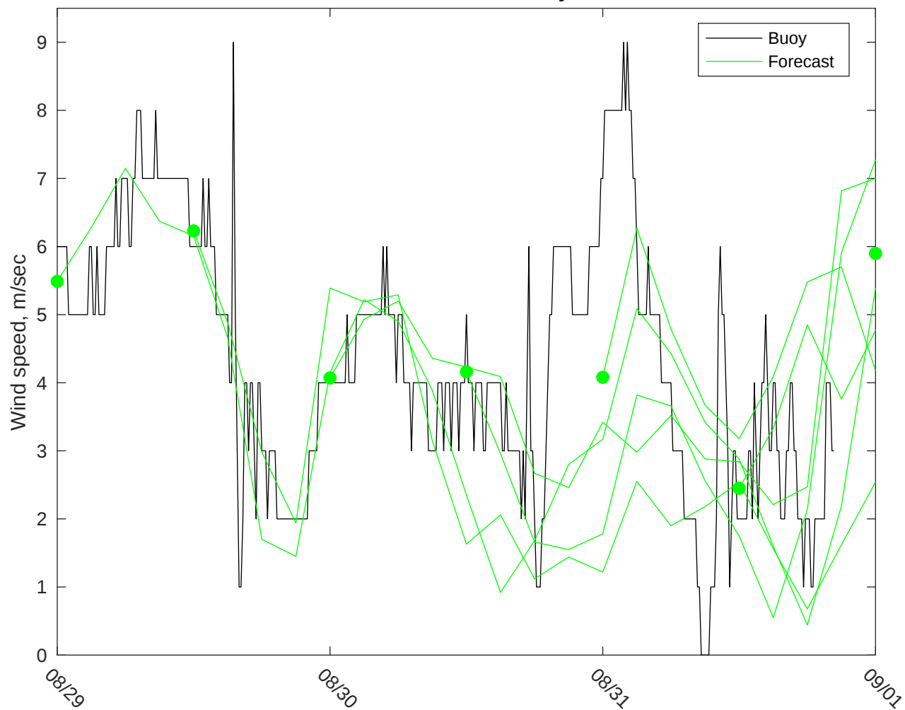
NDBC 42035 vs GFS Winds: 0 to 3 day forecast
