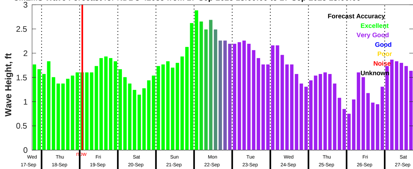
CMEMS Wave Forecast for NDBC 42035 from 17-Sep-2025 18:00:00 to 27-Sep-2025 18:00:00
