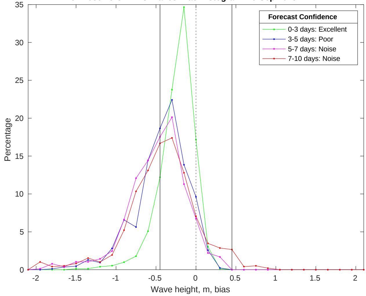
NDBC 42036 vs CMEMS Waves Bias Histogram: 19-Sep-2025
