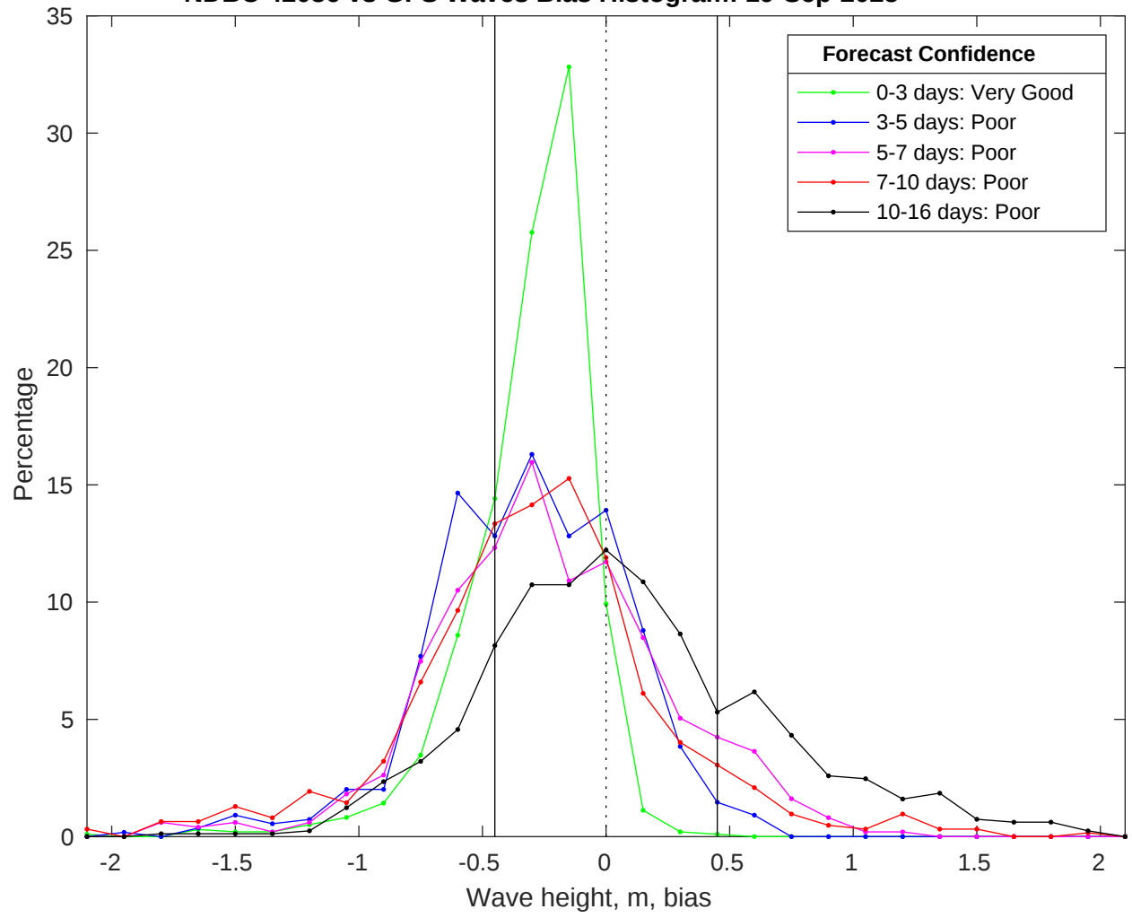
NDBC 42036 vs GFS Waves Bias Histogram: 19-Sep-2025
