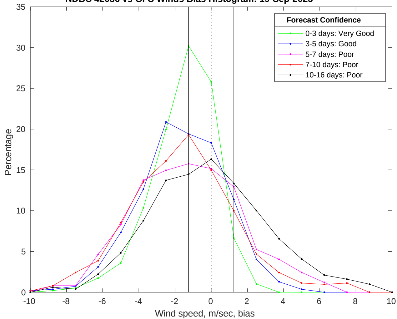
NDBC 42036 vs GFS Winds Bias Histogram: 19-Sep-2025
