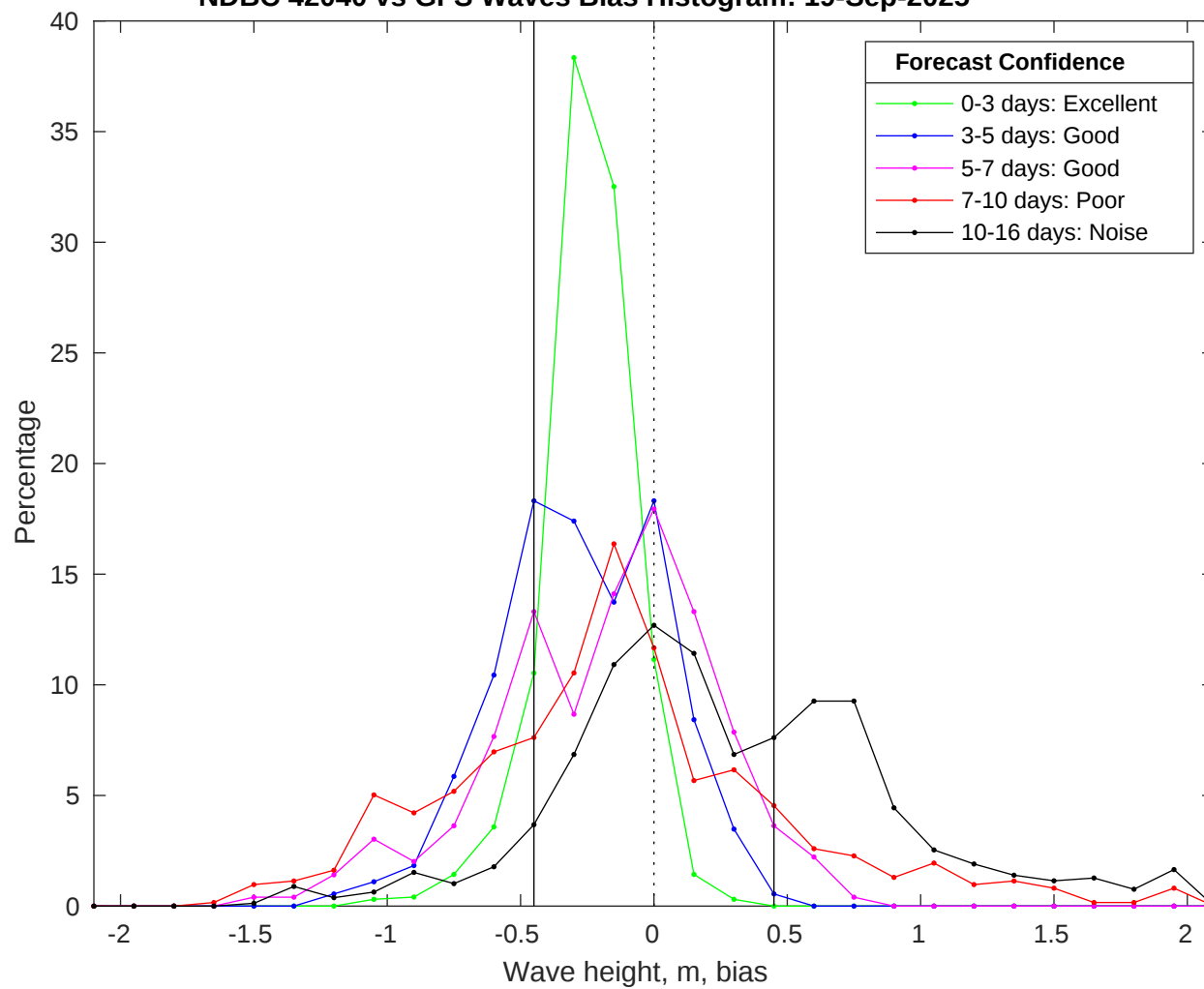
NDBC 42040 vs GFS Waves Bias Histogram: 19-Sep-2025
