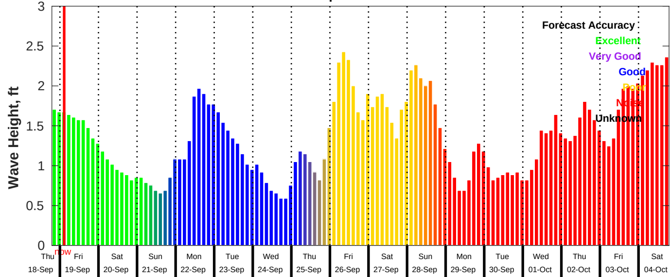
GFS Wave Forecast for NDBC 42040 from 18-Sep-2025 19:00:00 to 04-Oct-2025 19:00:00
