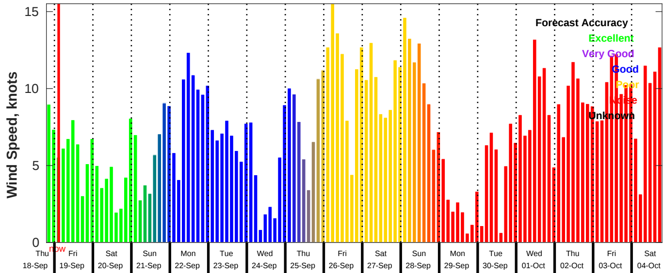
GFS Wind Speed Forecast for NDBC 42040 from 18-Sep-2025 19:00:00 to 04-Oct-2025 19:00:00
