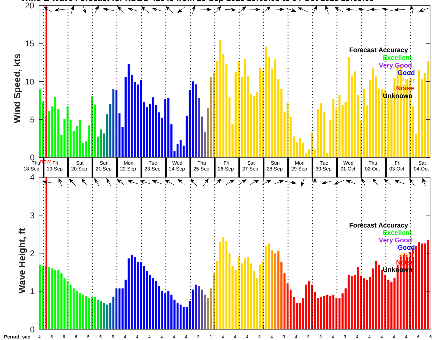
Wind & Wave Forecast for NDBC 42040 from 18-Sep-2025 19:00:00 to 04-Oct-2025 19:00:00
