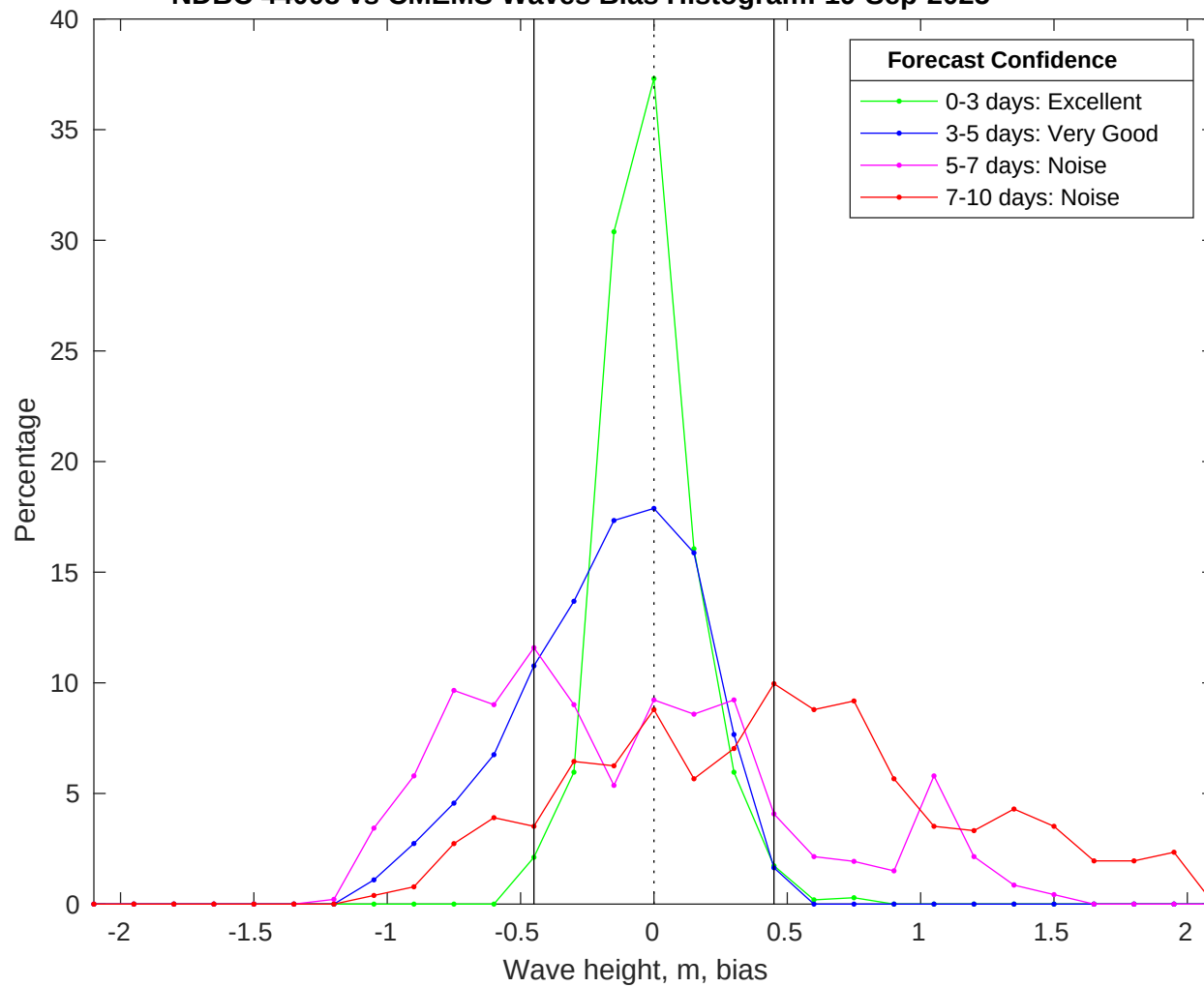
NDBC 44008 vs CMEMS Waves Bias Histogram: 19-Sep-2025
