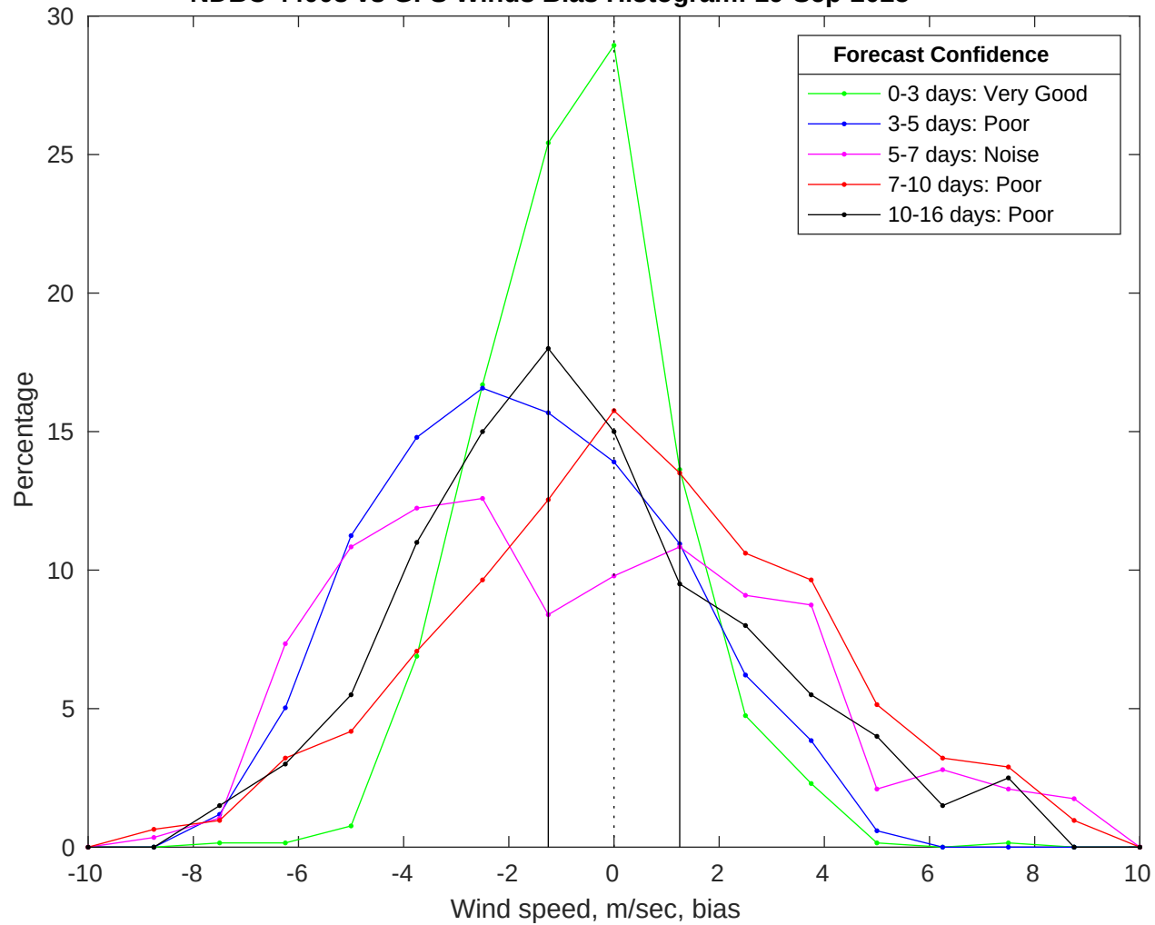
NDBC 44008 vs GFS Winds Bias Histogram: 19-Sep-2025
