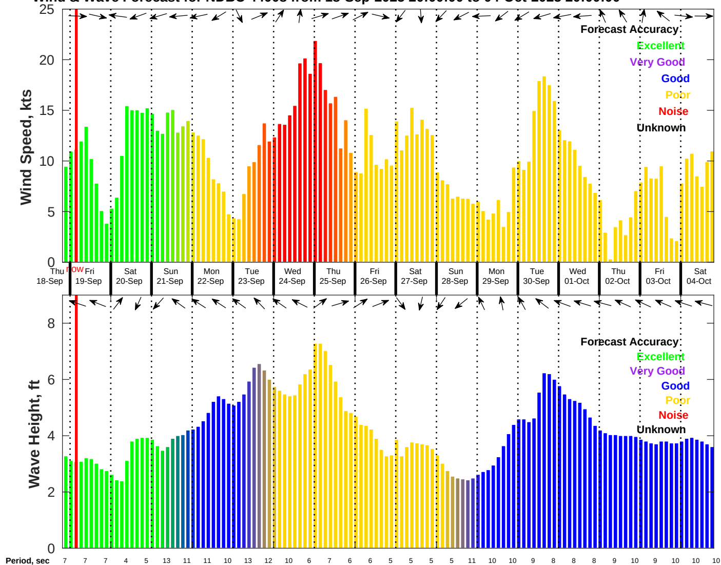
Wind & Wave Forecast for NDBC 44008 from 18-Sep-2025 20:00:00 to 04-Oct-2025 20:00:00
