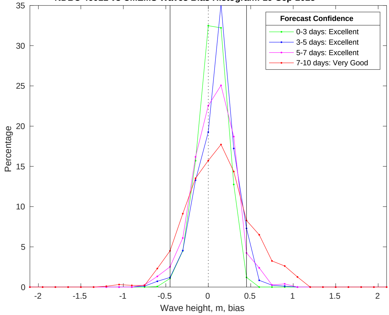
NDBC 46011 vs CMEMS Waves Bias Histogram: 19-Sep-2025
