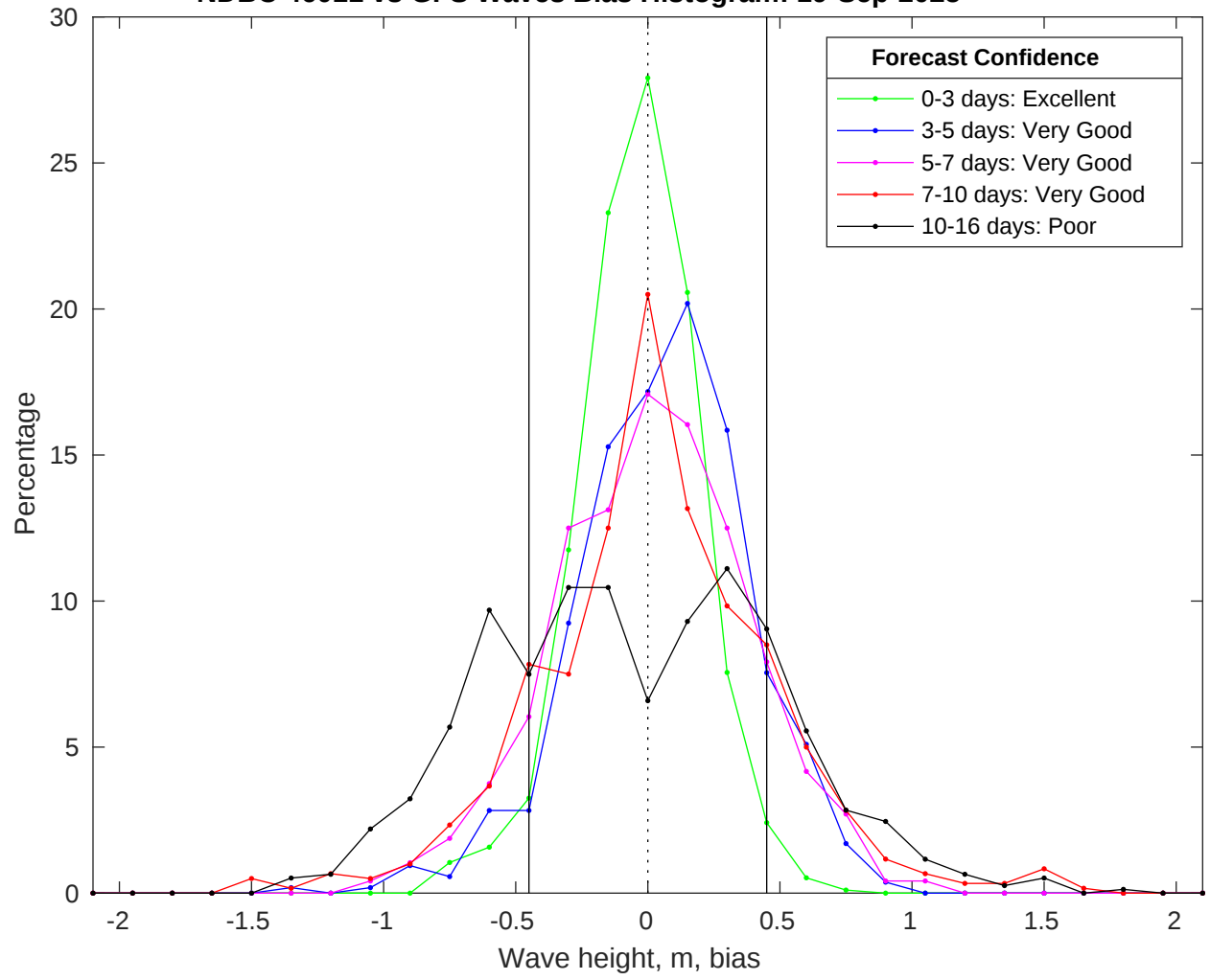
NDBC 46011 vs GFS Waves Bias Histogram: 19-Sep-2025
