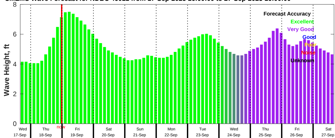
CMEMS Wave Forecast for NDBC 46011 from 17-Sep-2025 16:00:00 to 27-Sep-2025 16:00:00
