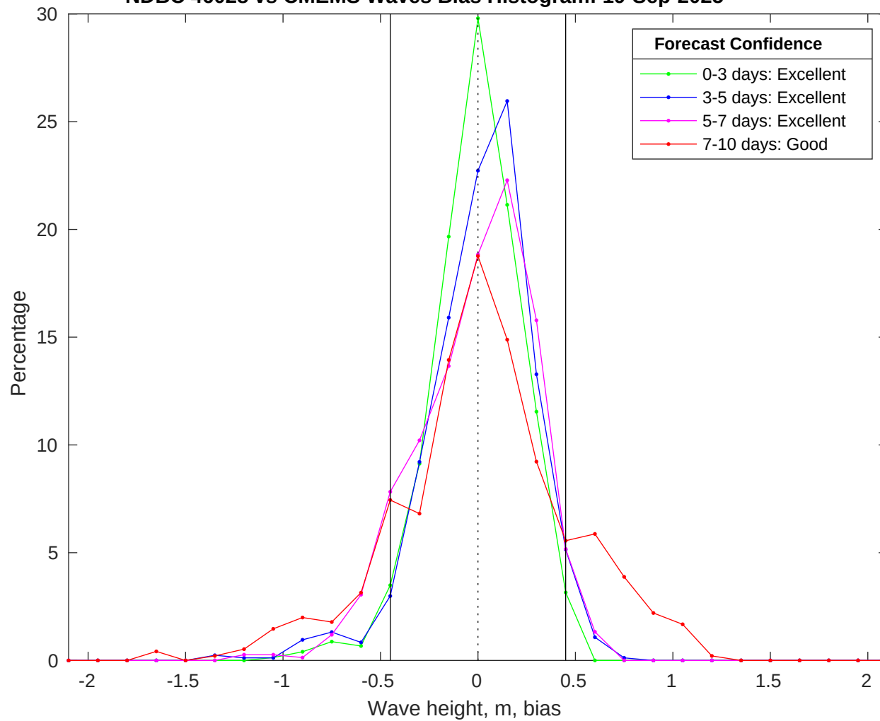
NDBC 46028 vs CMEMS Waves Bias Histogram: 19-Sep-2025
