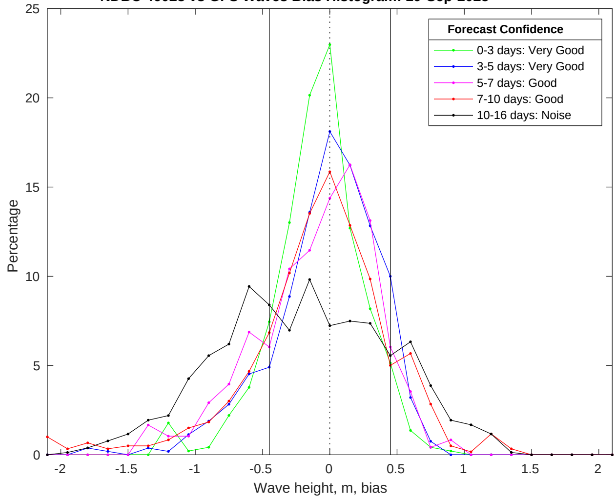
NDBC 46028 vs GFS Waves Bias Histogram: 19-Sep-2025
