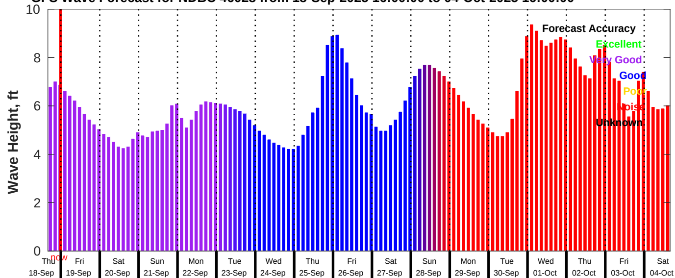
GFS Wave Forecast for NDBC 46028 from 18-Sep-2025 16:00:00 to 04-Oct-2025 16:00:00
