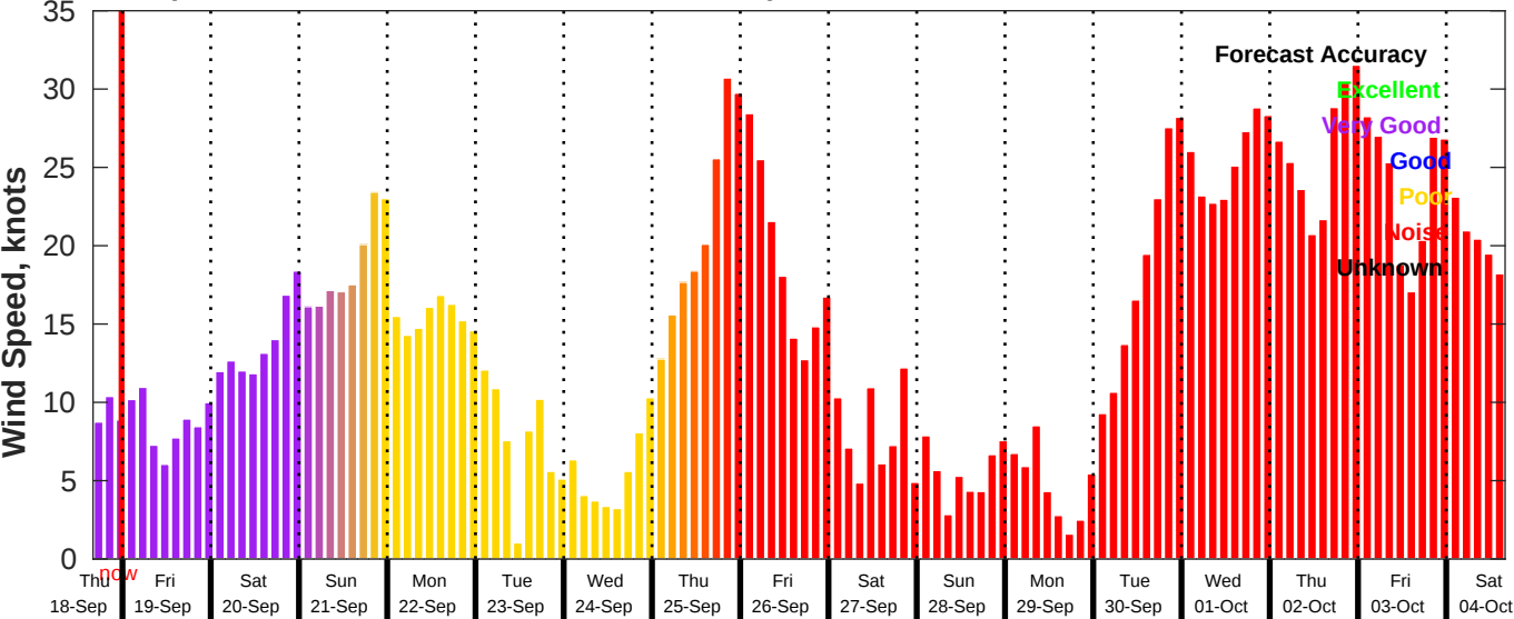
GFS Wind Speed Forecast for NDBC 46028 from 18-Sep-2025 16:00:00 to 04-Oct-2025 16:00:00
