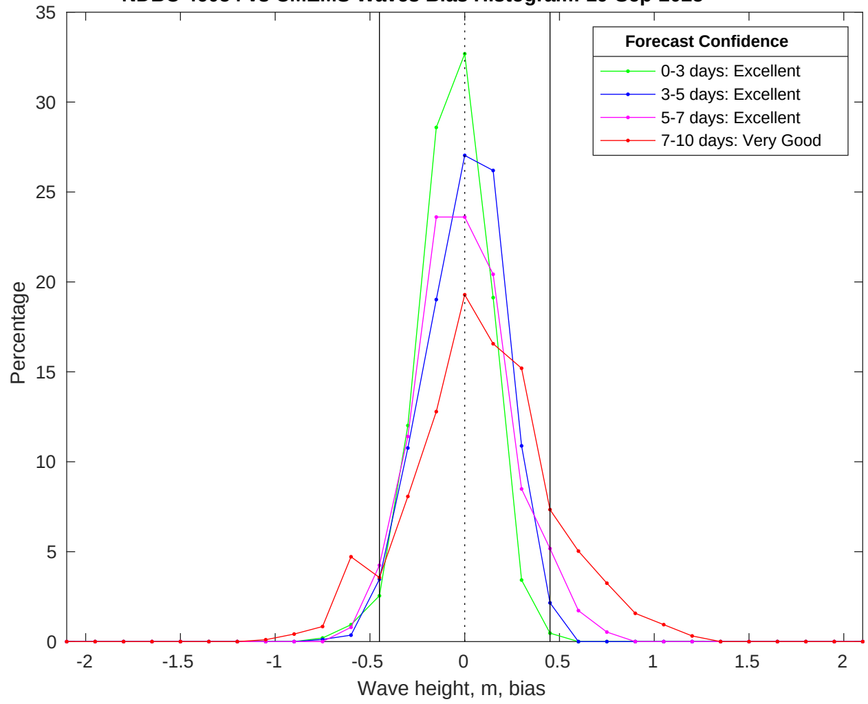
NDBC 46054 vs CMEMS Waves Bias Histogram: 19-Sep-2025
