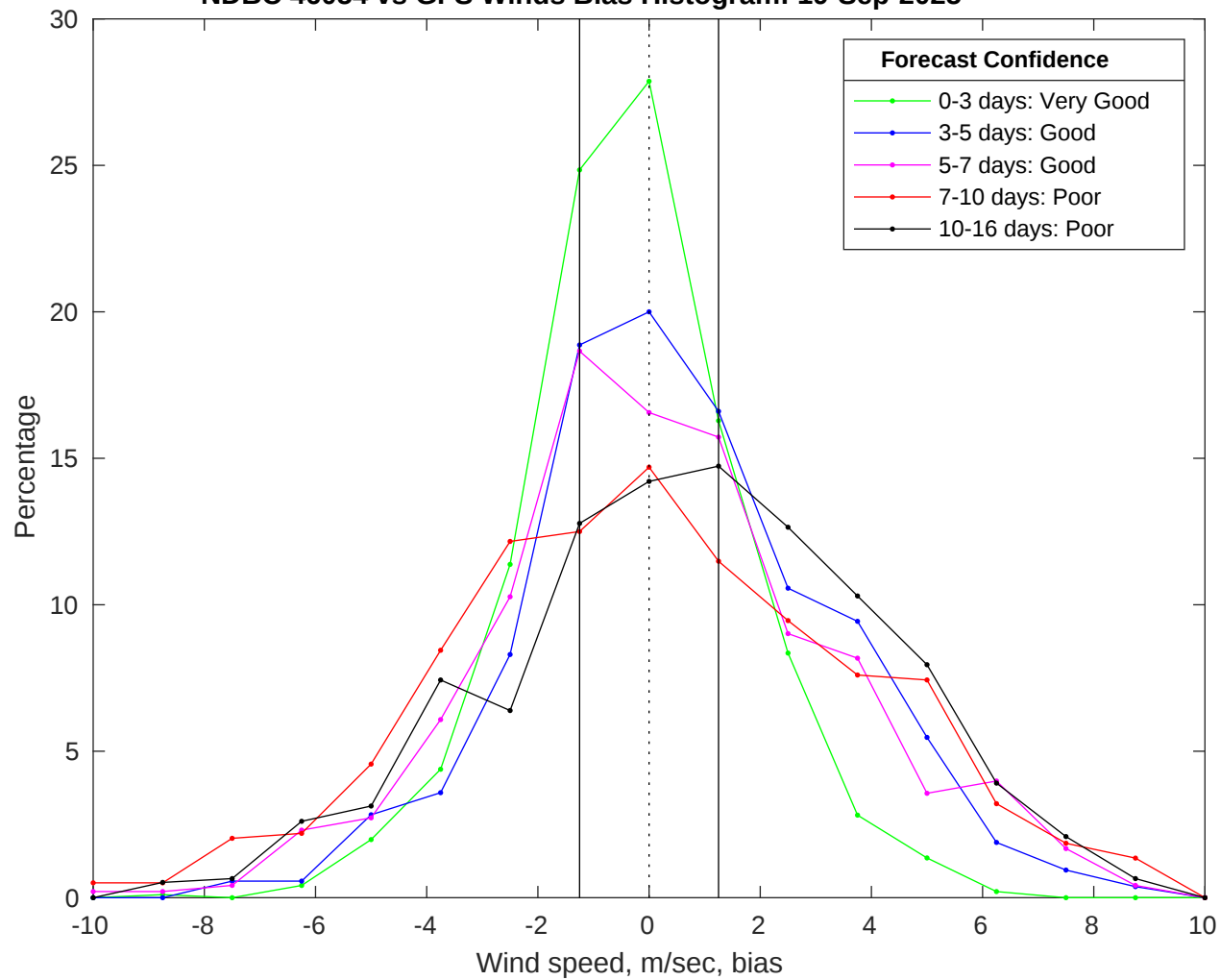
NDBC 46054 vs GFS Winds Bias Histogram: 19-Sep-2025
