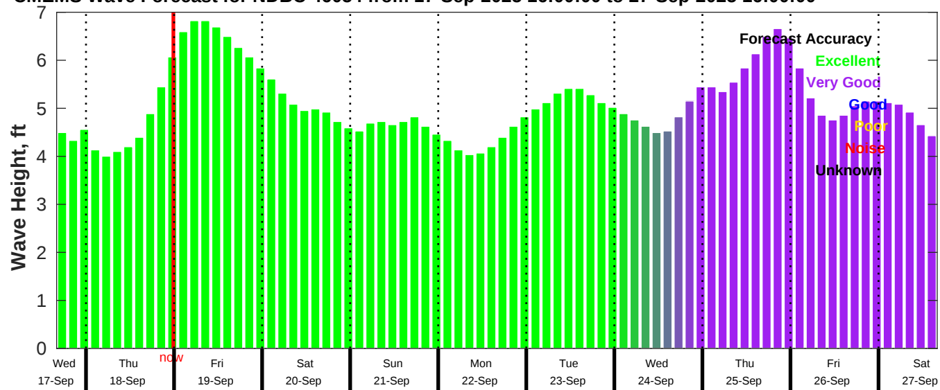
CMEMS Wave Forecast for NDBC 46054 from 17-Sep-2025 16:00:00 to 27-Sep-2025 16:00:00
