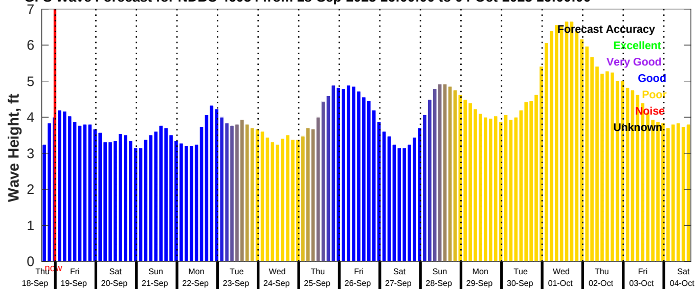
GFS Wave Forecast for NDBC 46054 from 18-Sep-2025 16:00:00 to 04-Oct-2025 16:00:00
