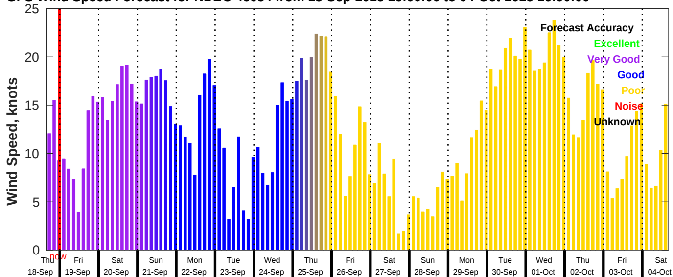
GFS Wind Speed Forecast for NDBC 46054 from 18-Sep-2025 16:00:00 to 04-Oct-2025 16:00:00
