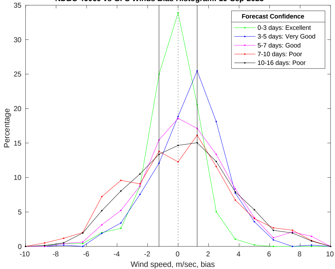
NDBC 46069 vs GFS Winds Bias Histogram: 19-Sep-2025
