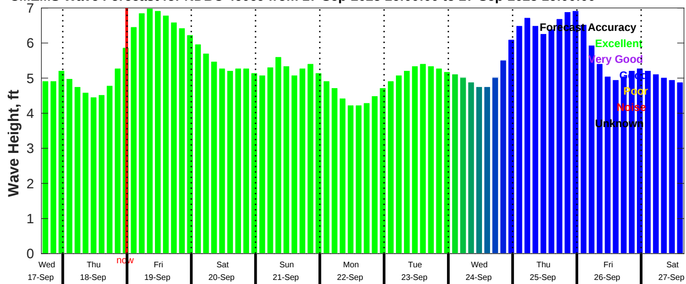
CMEMS Wave Forecast for NDBC 46069 from 17-Sep-2025 16:00:00 to 27-Sep-2025 16:00:00
