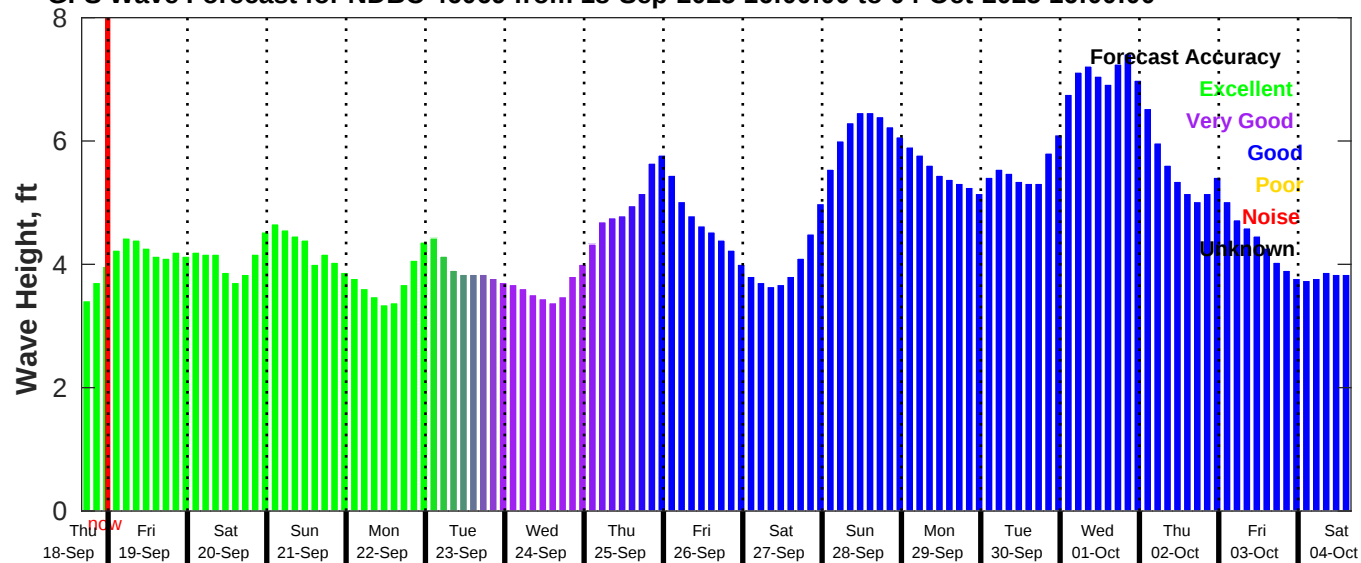
GFS Wave Forecast for NDBC 46069 from 18-Sep-2025 16:00:00 to 04-Oct-2025 16:00:00
