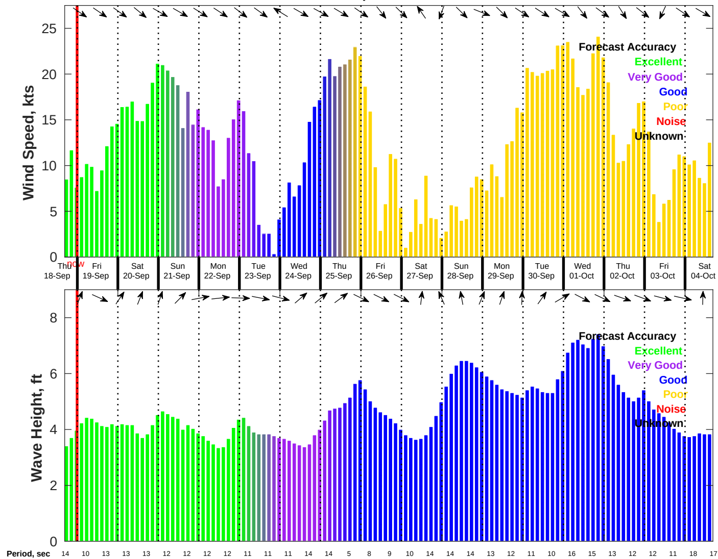
Wind & Wave Forecast for NDBC 46069 from 18-Sep-2025 16:00:00 to 04-Oct-2025 16:00:00
