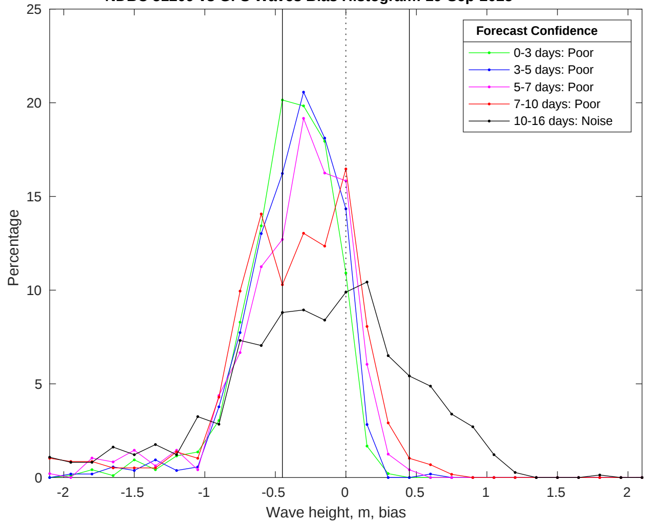
NDBC 51209 vs GFS Waves Bias Histogram: 19-Sep-2025
