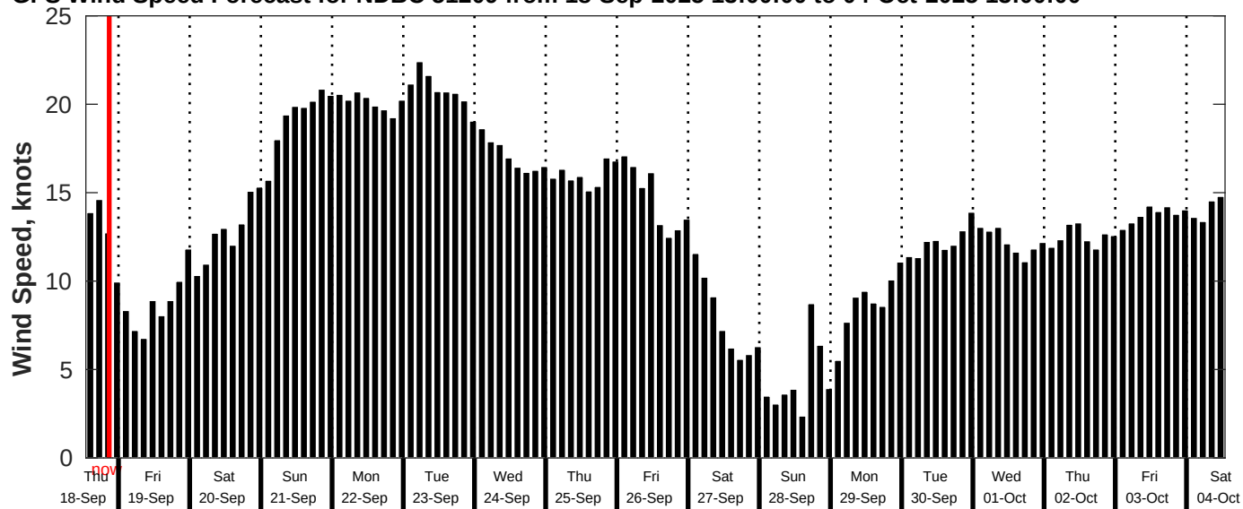
GFS Wind Speed Forecast for NDBC 51209 from 18-Sep-2025 13:00:00 to 04-Oct-2025 13:00:00
