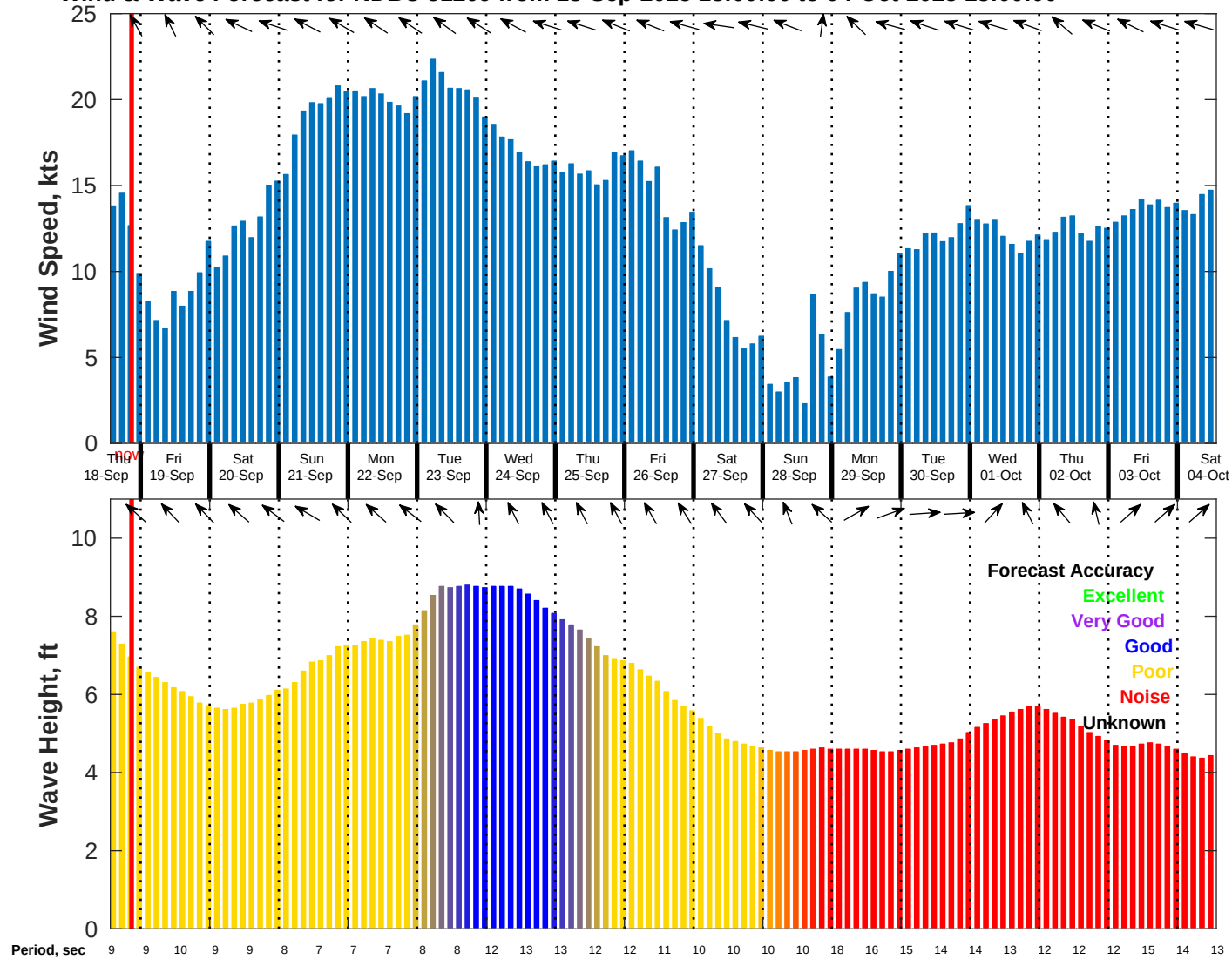
Wind & Wave Forecast for NDBC 51209 from 18-Sep-2025 13:00:00 to 04-Oct-2025 13:00:00
