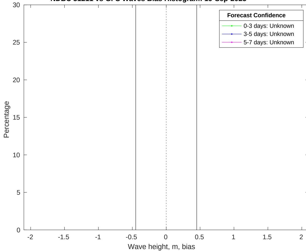
NDBC 51211 vs GFS Waves Bias Histogram: 19-Sep-2025
