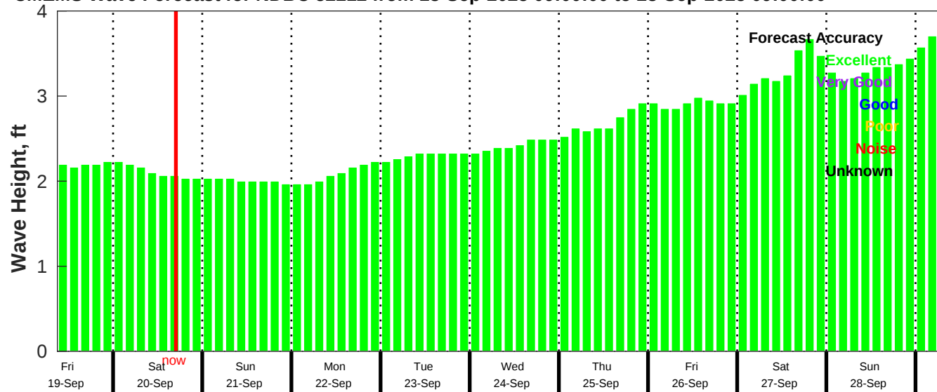
CMEMS Wave Forecast for NDBC 52212 from 18-Sep-2025 09:00:00 to 28-Sep-2025 09:00:00
