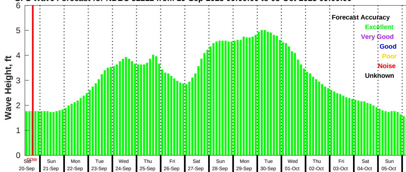
GFS Wave Forecast for NDBC 52212 from 19-Sep-2025 09:00:00 to 05-Oct-2025 09:00:00
