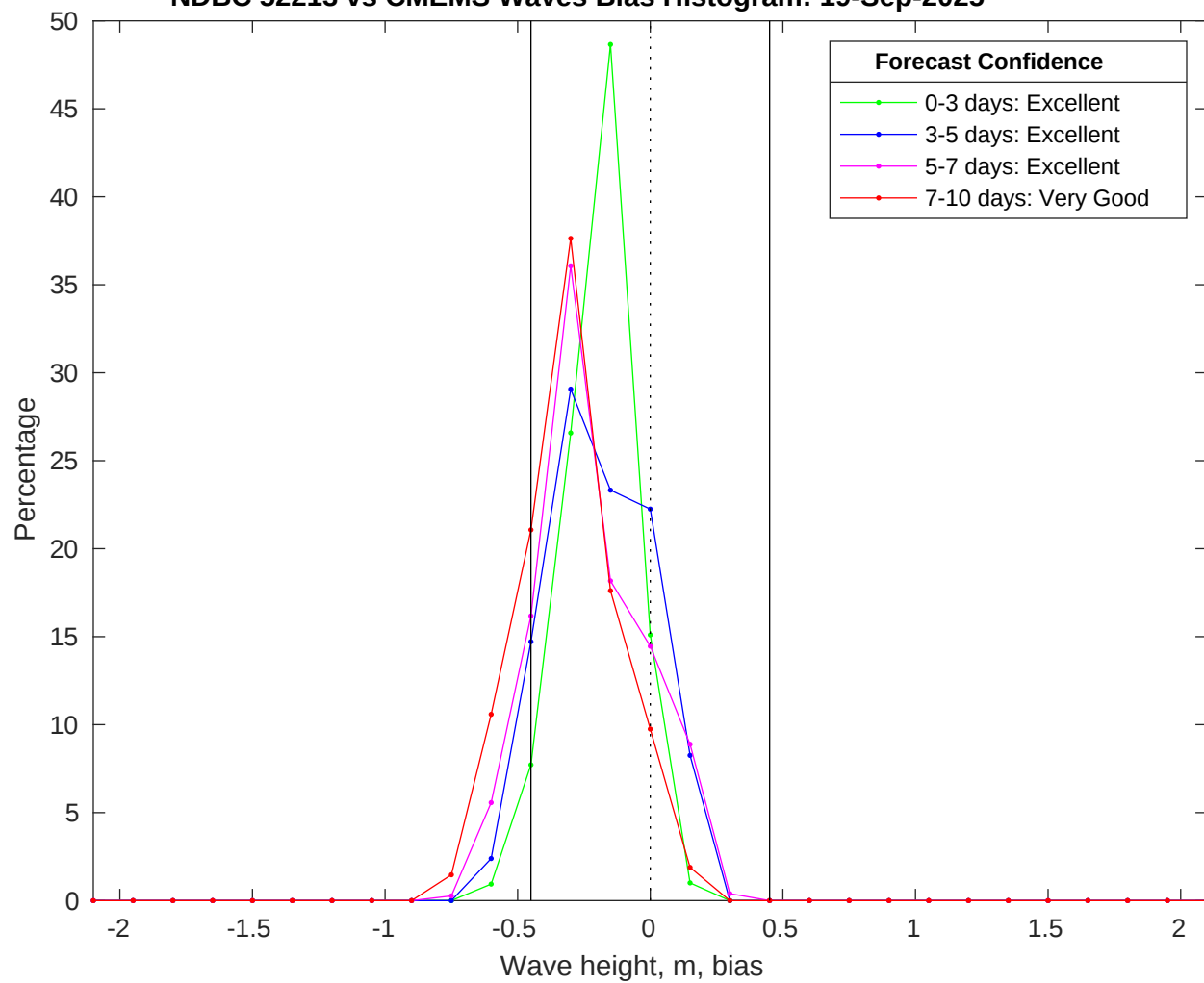
NDBC 52213 vs CMEMS Waves Bias Histogram: 19-Sep-2025
