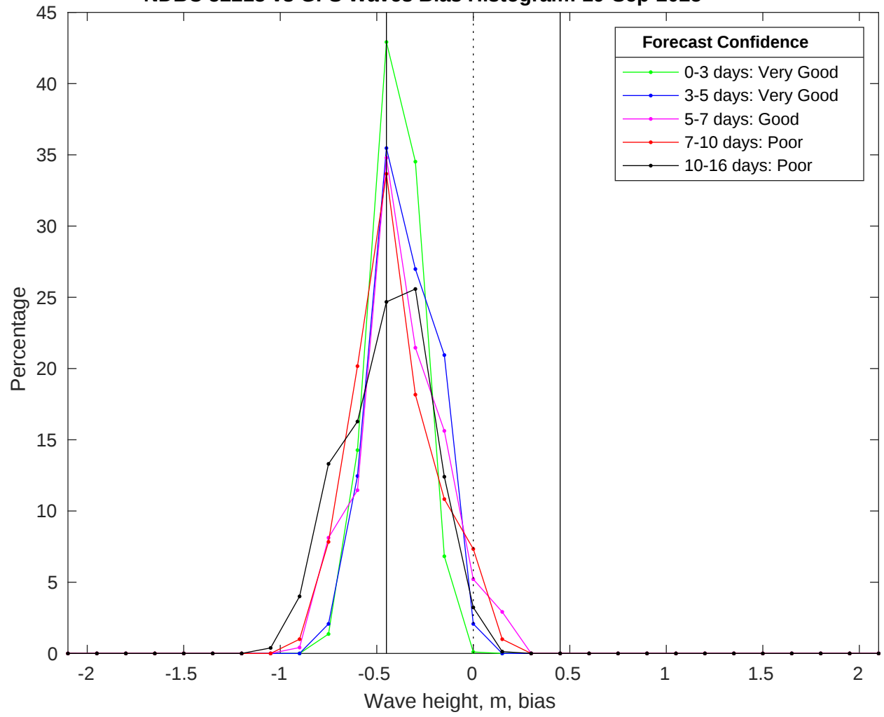
NDBC 52213 vs GFS Waves Bias Histogram: 19-Sep-2025
