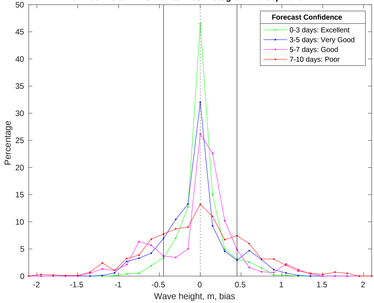
NDBC 41004 vs CMEMS Waves Bias Histogram: 20-Sep-2025
